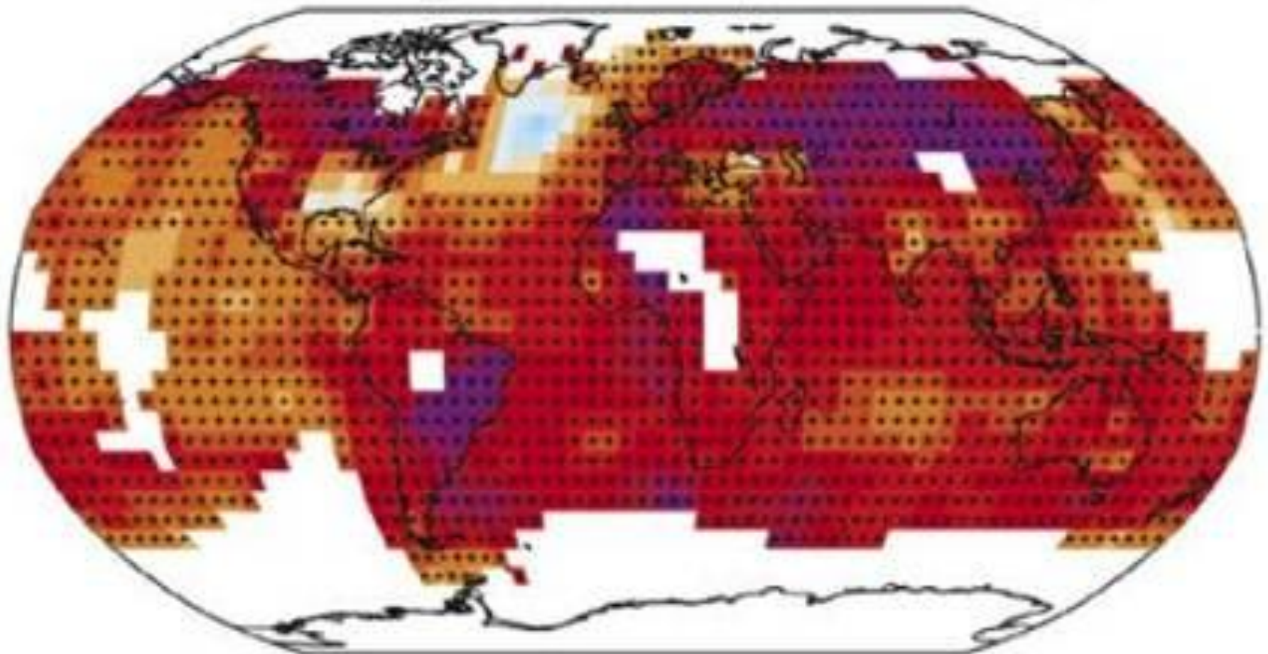
Observed change in surface temperature 1901–2012
